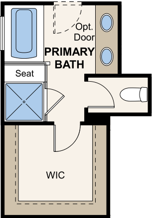
OPT. PRIMARY BATH TUB & SHOWER
